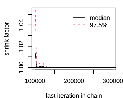
d.chemo.Afatinib
